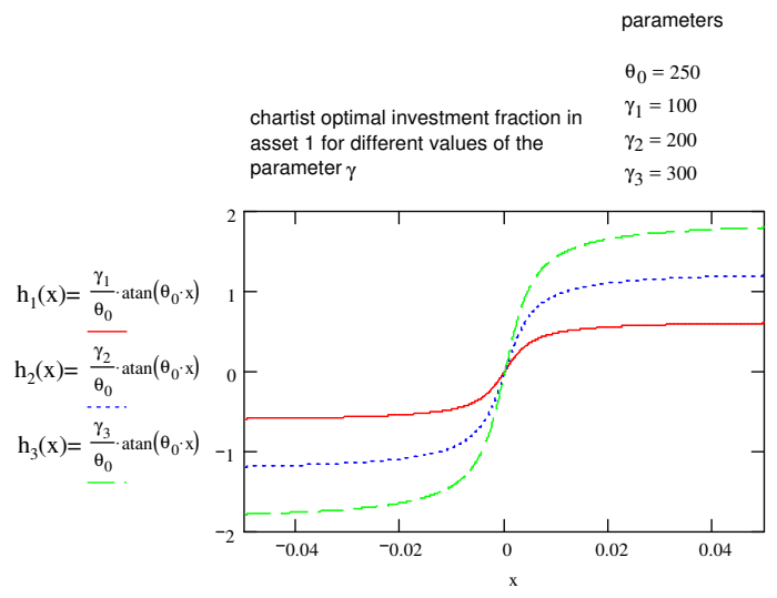
Figure 1: chartist demand function.
