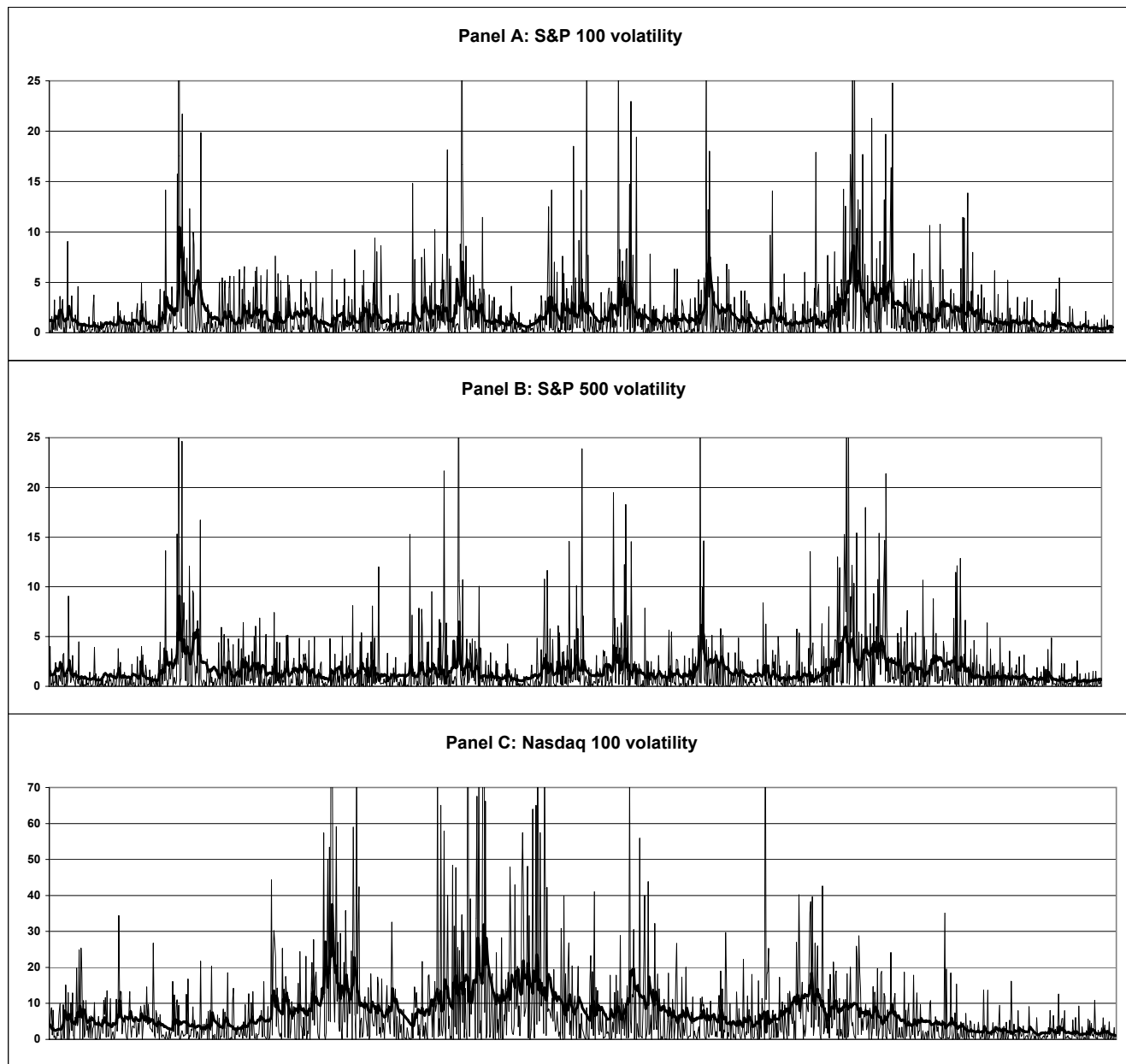
Figure 1: Realized and forecast volatility from Model 4
